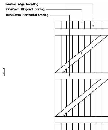
1.8m HIGH TIMBER GATE
