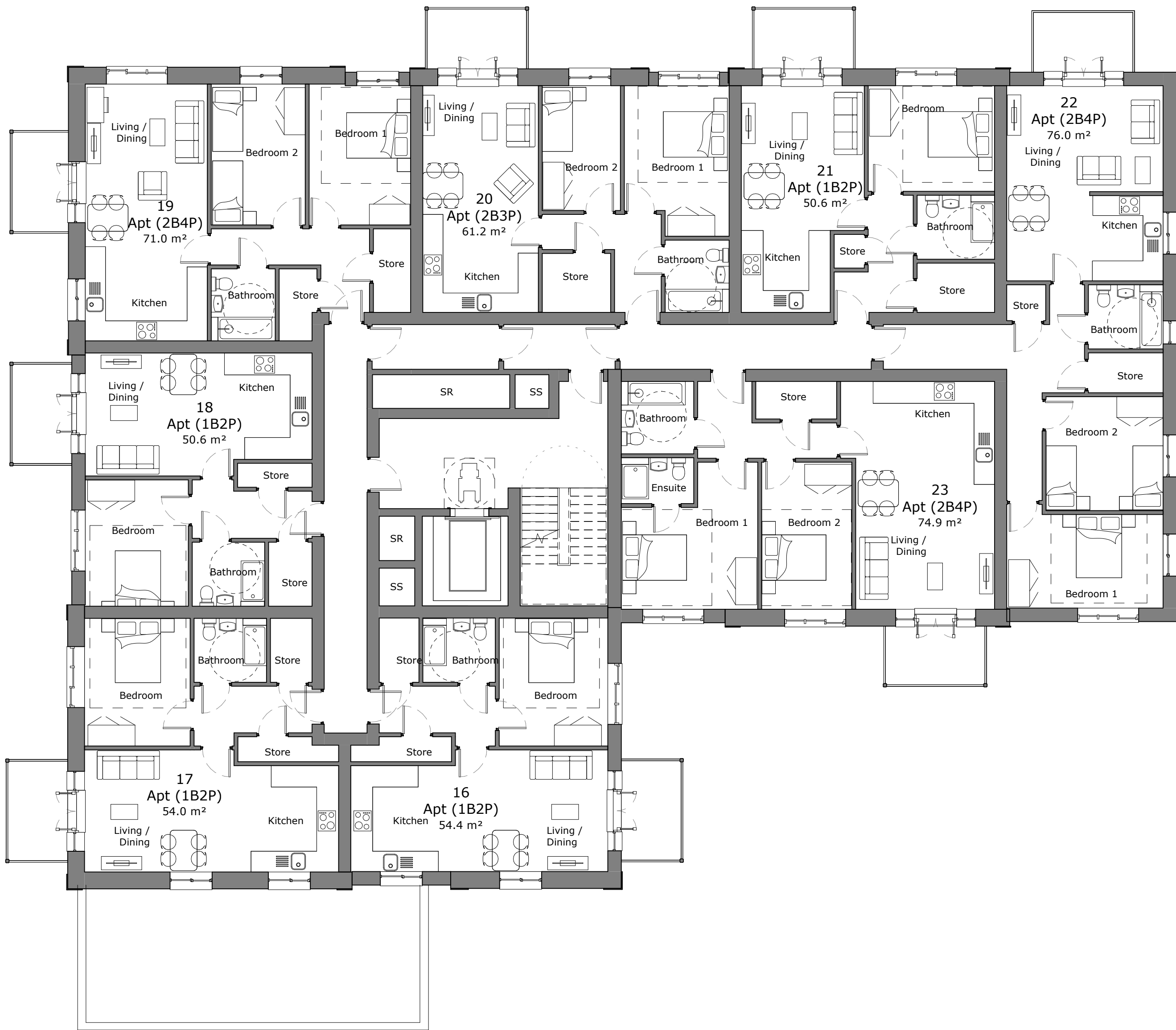
2nd Floor 1 : 100
