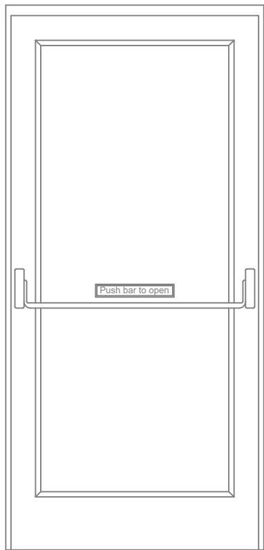
Door A Existing Internal Elevations
